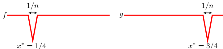
Fig. 1. f is uniform everywhere except a small neighbourhood around 1/4 where it has a sharp ‘v’ shape. And g is the reflection of f about x = 1/2 .
